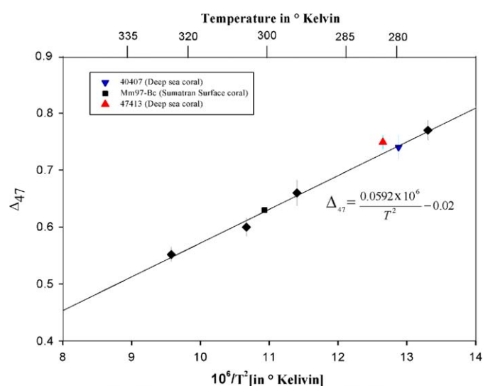
Fig. 5. Values of \Delta_{47} of \text{CO}_2 extracted from calcites grown from aqueous solution (reproduced from Fig. 4) and of deep-sea and surface corals, plotted vs. 10^6/T^2 , where T is the known growth temperature in Kelvin. Note that both surface and deep-sea aragonitic corals generally conform to the trend defined by inorganic calcites. Deep-sea coral 47413 lies slightly ( 0.02\text{‰} ) above this trend, perhaps suggesting a subtle ‘vital effect’ (this aliquot of this sample exhibits extreme vital effects on its \delta^{13}\text{C} and \delta^{18}\text{O} values; Table 5).
