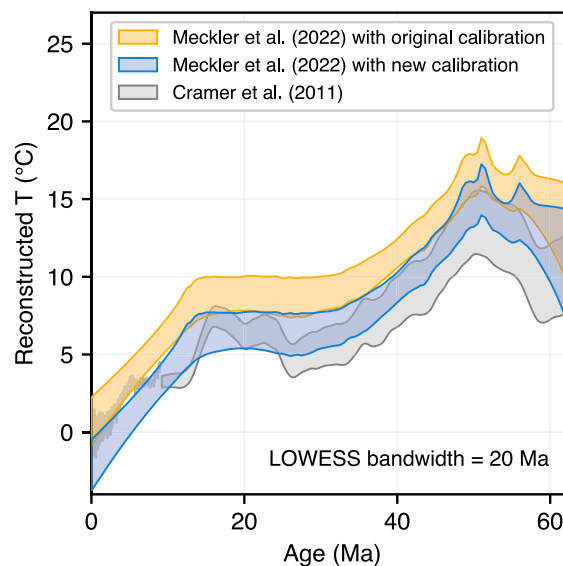
Figure 18. Comparison of smoothed reconstructions of deep ocean temperature. In gray: 90% confidence band of T_{18} reconstructed by Cramer et al. (2011). In yellow: 95% confidence band of a LOWESS regression of the Meckler et al. (2022) data, converted to T_{47} using the Meinicke et al. (2021) calibration. In blue: 95% confidence band of a LOWESS regression of the same data, but converted to T_{47} using our new planktic calibration (Equation 5). The LOWESS bandwidth was chosen arbitrarily to yield approximately the same width and level of detail as the Cramer et al. (2011) reconstruction. LOWESS 95% confidence limits are estimated using a quasi-Monte Carlo simulation where we quasi-randomly generate 2^{13} versions of the T_{47} data set.
