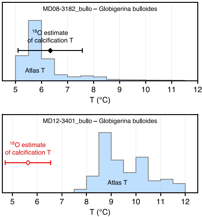
Figure 6. Planktic samples are categorized as concordant (top panel) or discordant (bottom panel) depending on whether the oxygen-18 estimate of their calcification temperature (red or black 95% error bar) overlaps with the seasonal distribution of temperatures (blue histogram) in the assumed calcification depth range for that species.
