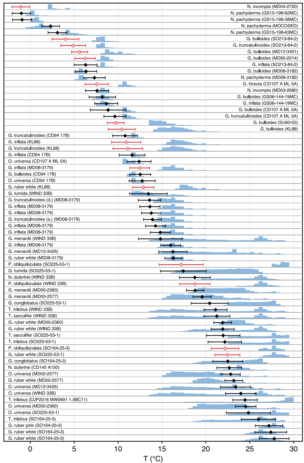
Figure 7. Comparison, for each planktic sample from Peral et al. (2018) and Meinicke et al. (2020), between oxygen-18 estimates of calcification temperatures (95% error bars) and year-long distribution (blue histograms) of monthly mean temperatures over the assumed living depth interval. T_{18} error bars for concordant and discordant samples are shown in black or red, respectively.
