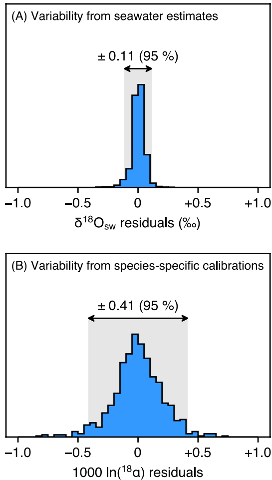
Figure 4. Sources of uncertainty affecting the use of oxygen-18 thermometry to constrain planktic foraminifer calcification temperatures. (a) Overall residuals for the depth- and month-integrated \delta^{18}\text{O}_{\text{sw}} values used to estimate seawater oxygen-18 composition for each planktic foraminifer sample. (b) Overall residuals for the species-specific oxygen-18 relationships listed in Table 4, based on all studies shown in Figure 3.
