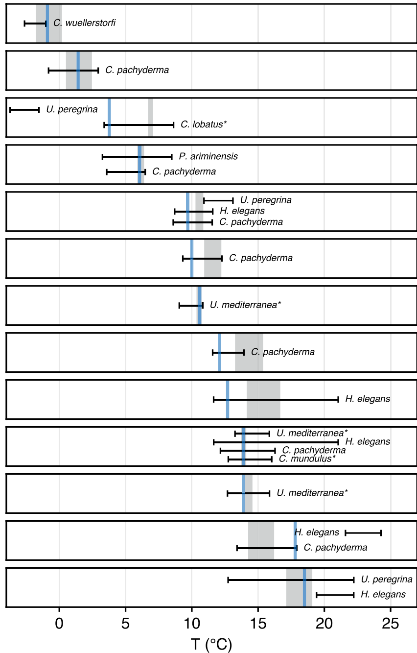
Figure 9. Comparison, for each benthic sample from Peral et al. (2018) and Piasecki et al. (2019), between oxygen-18 estimates of calcification temperatures (95% error bars), bottom mean annual temperatures (95% gray shading), and originally reported calcification temperatures (blue lines). Species listed with asterisks are those without direct observations constraining ^{18}\alpha .
