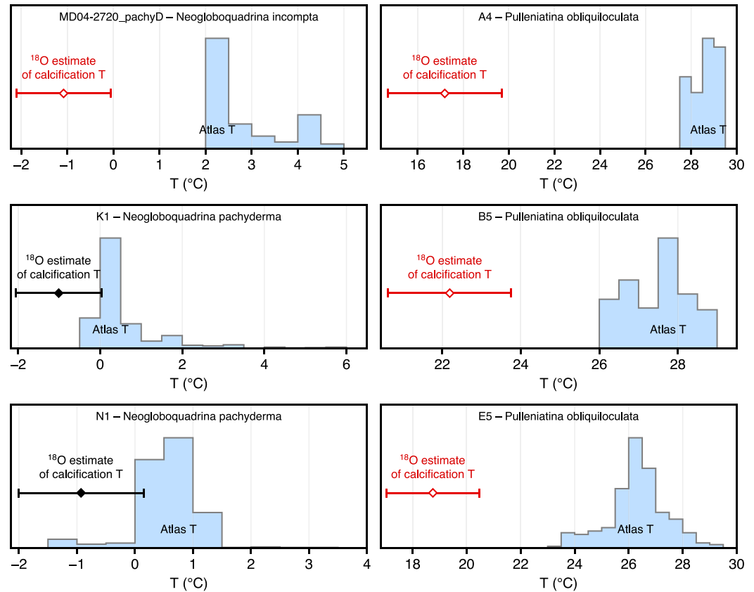
Figure 15. Comparison between oxygen-18 estimates of calcification temperatures (95% error bars) and year-long distribution (blue histograms) of monthly mean temperatures over the assumed living depth interval for the three coldest planktic samples (left column, see Section 3.2.2) and the P. obliquiloculata samples (right column, see Section 3.4.3).
