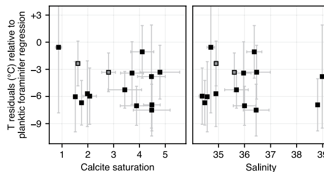
Figure 14. The benthic residuals of Figure 13 are not obviously correlated with seawater chemistry. Calcite saturation and salinity were estimated from GLODAPv2 (Lauvset et al., 2016).
