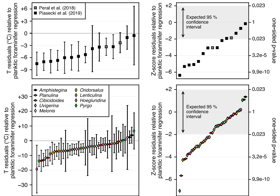
Figure 13. Temperature residuals (left panels) and corresponding Z-scores (right panels) for benthic samples from Peral et al. (2018) and Piasecki et al. (2019), relative to the planktic regression of Equation 5. Top row: results averaged by core top. Bottom row: results averaged by species at each core top. Vertical and horizontal diamonds represent infaunal and epifaunal species, respectively. Colored markers correspond to different genera. The right axis in each of right panels indicates the p-values corresponding to Z-scores for a Gaussian distribution.
