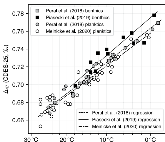
Figure 2. Foraminifer calibration data sets as originally published. Different studies used different methods to estimate calcification temperatures (see Section 2.3.1). \Delta_{47} values are standardized using the same set of reference materials but correspond to the “historical” CDES scale (Dennis et al., 2011).
