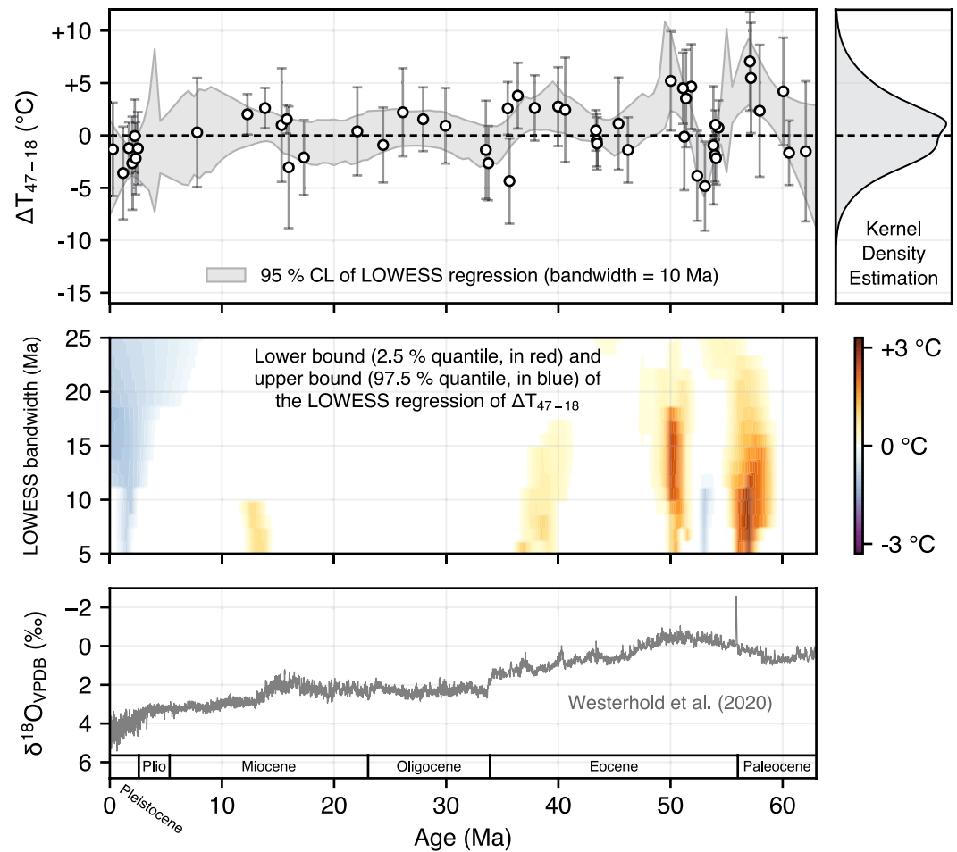
Figure 17. Top left: plot of \Delta T_{47-18} , defined as the difference between the benthic T_{47} values of Meckler et al. (2022), reprocessed using this study's planktic regression (Equation 5), and the corresponding \delta^{18}O_c -derived T_{18} record from Cramer et al. (2011). Vertical error bars account for estimated analytical and calibration errors on \Delta_{47} as well as the originally reported T_{18} uncertainties. Green shaded area is the central 95% confidence band for a LOWESS regression of \Delta T_{47-18} with a bandwidth equal to 10 Ma. Top right: kernel density estimation for the whole (unsmoothed) data set, showing that the long-term average of \Delta T_{47-18} is close to zero. Center panel: white areas correspond to periods when \Delta T_{47-18} does not significantly differ from zero, and shaded areas to periods when T_{47} is significantly warmer (in red) or colder (in blue) than T_{18} at the 95% confidence level, with color density corresponding to the 2.5% and 97.5% quantiles, respectively, of (T_{47} - T_{18}) . Note that color densities conservatively denote the minimum level of mismatch (at 95% confidence); average values of smoothed \Delta T_{47-18} are further away from zero. Bottom panel: smoothed benthic \delta^{18}O_c record of Westerhold et al. (2020).
