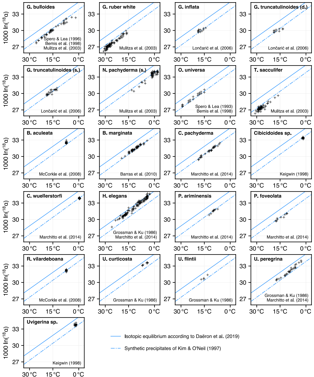
Figure 3. Constraints linking ^{18}\alpha to calcification temperatures for species listed in Table 2. Although these fractionation relationships differ between species, their temperature sensitivities remain indistinguishable from that for inorganic calcite (blue lines). All temperatures observations are from the original studies.
