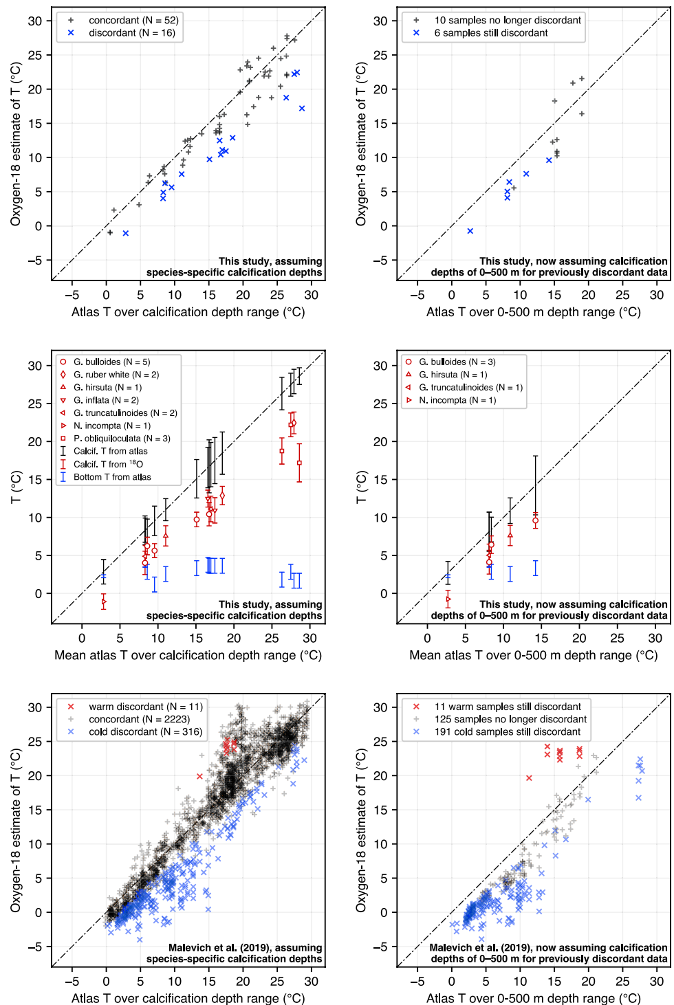
Figure 8. Distribution of discordant samples in our clumped-isotope data set (Peral et al., 2018; Meinicke et al., 2020, top two rows) and in a much larger compilation of Holocene core tops (Malevich et al., 2019, bottom row). Top row: T_{18} versus atlas temperatures over assumed living depth range (left panel) or over 0–500 m (right panel) for the clumped-isotope data set. Center row: Comparison of T_{18} with local bottom ocean temperatures and with atlas temperatures over assumed living depth range (left panel) or over 0–500 m (right panel) for the clumped-isotope data set. Bottom row: T_{18} versus atlas temperatures over assumed living depth range (left panel) or over 0–500 m (right panel) for the Malevich et al. data set. Right panel in each row only shows previously discordant samples.
