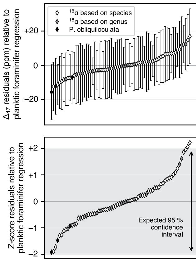
Figure 12. Regression residuals for the planktic samples from Peral et al. (2018) and Meinicke et al. (2020). Error bars in top panel are with 95% confidence limits from combined uncertainties in \Delta_{47} and calcification temperatures. Z-scores in bottom panel are computed based on these same error bars.
